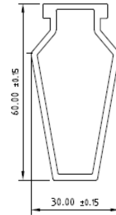
Truncated Fin Profile 30 x 60 mm
